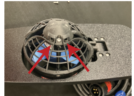
For Transducer Mounted Models
